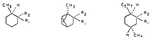
Ia R_1 = \text{NH}_2, R_2 = \text{H} IIa R_1 = \text{NH}_2, R_2 = \text{H} IIIa R_1 = \text{NH}_2, R_2 = \text{H} Ib R_1 = \text{H}, R_2 = \text{NH}_2 IIb R_1 = \text{H}, R_2 = \text{NH}_2 IIIb R_1 = \text{H}, R_2 = \text{NH}_2
